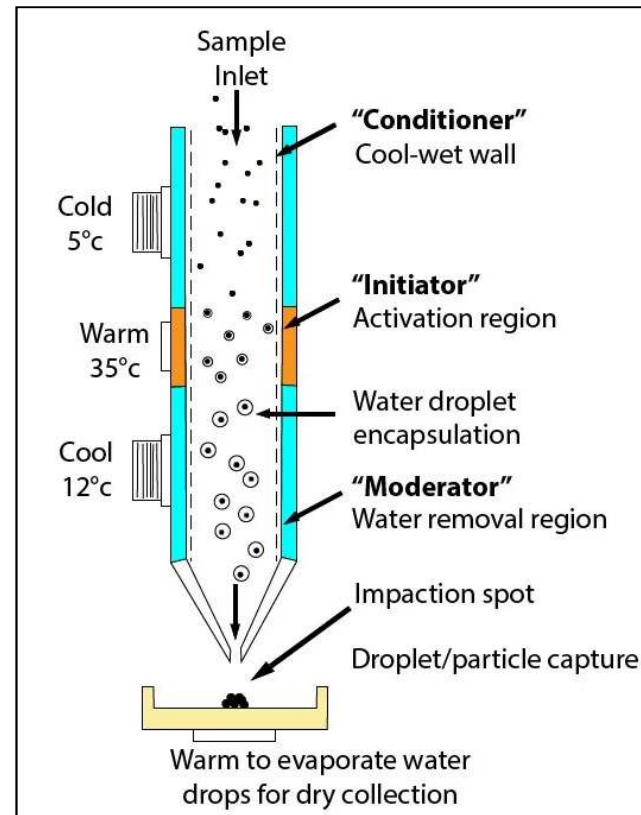
Aerosol Devices Model SSS110 Sequential Spot Sampler
