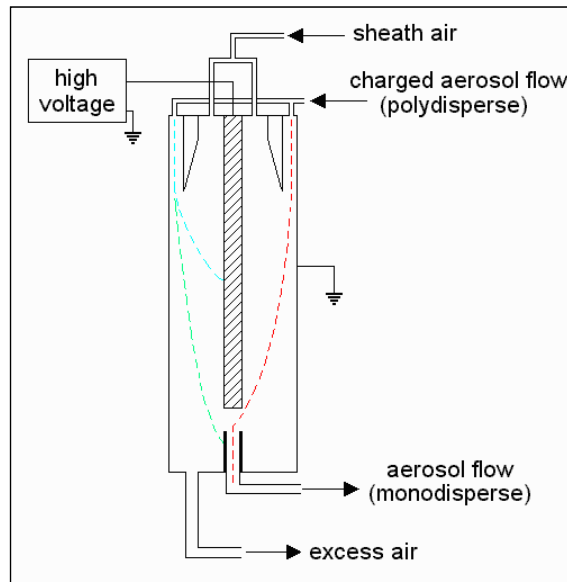
Differential Mobility Analyzer (DMA)
