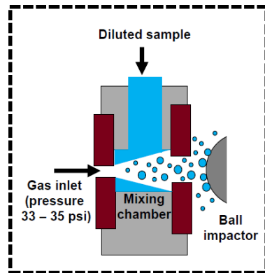
Kanomax FMT NanoParticle Nebulizer Model 9110
