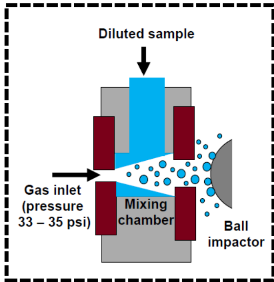
Precision Nebulizer
