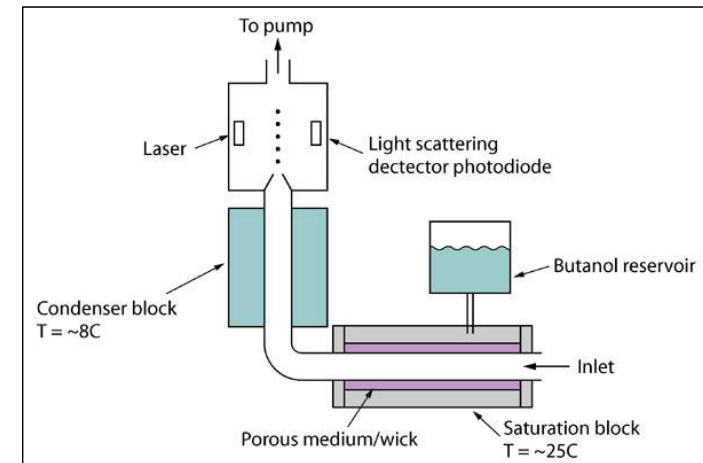
Condensation Particle Counter (CPC)
